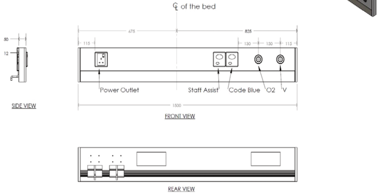
Systemz Modular Bedhead Panel (Single Channel)
