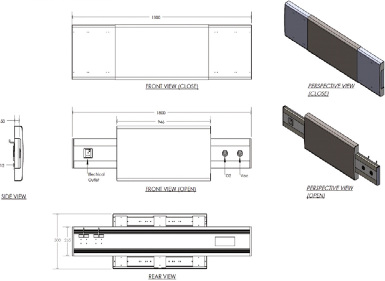
Systemz Modular Bedhead Panel With Sliding Panels(Single Channel)
