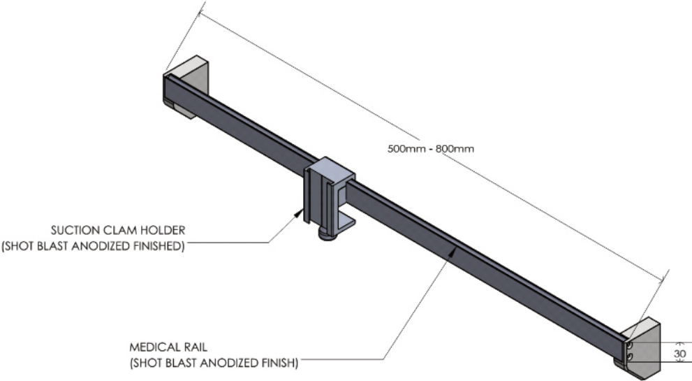
Standalone Medical Rail & Suction Clam Holder
